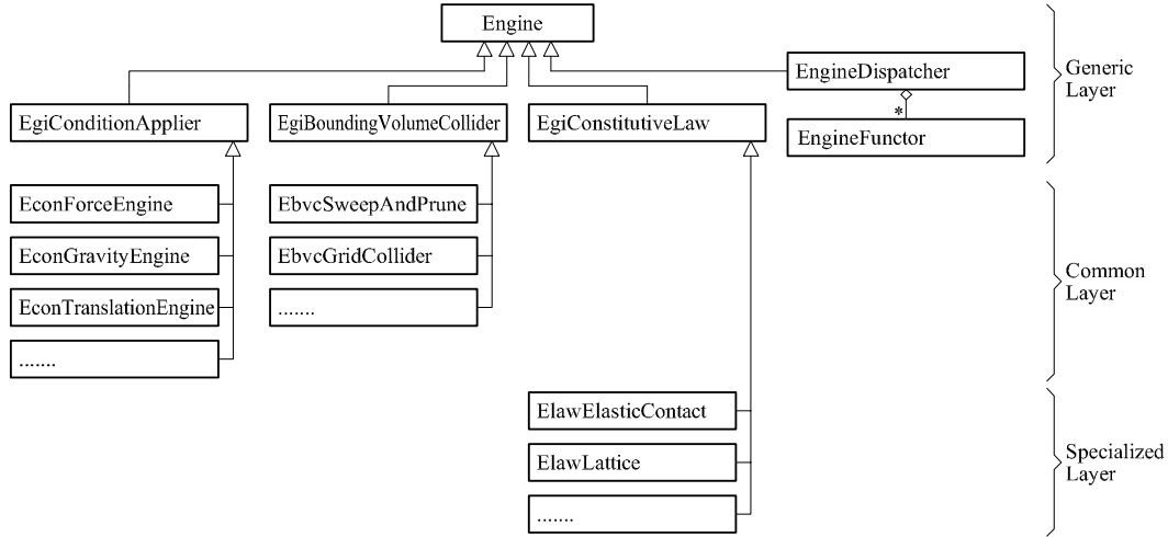
Fig. 14. Class Engine and example algorithms inheriting from it
