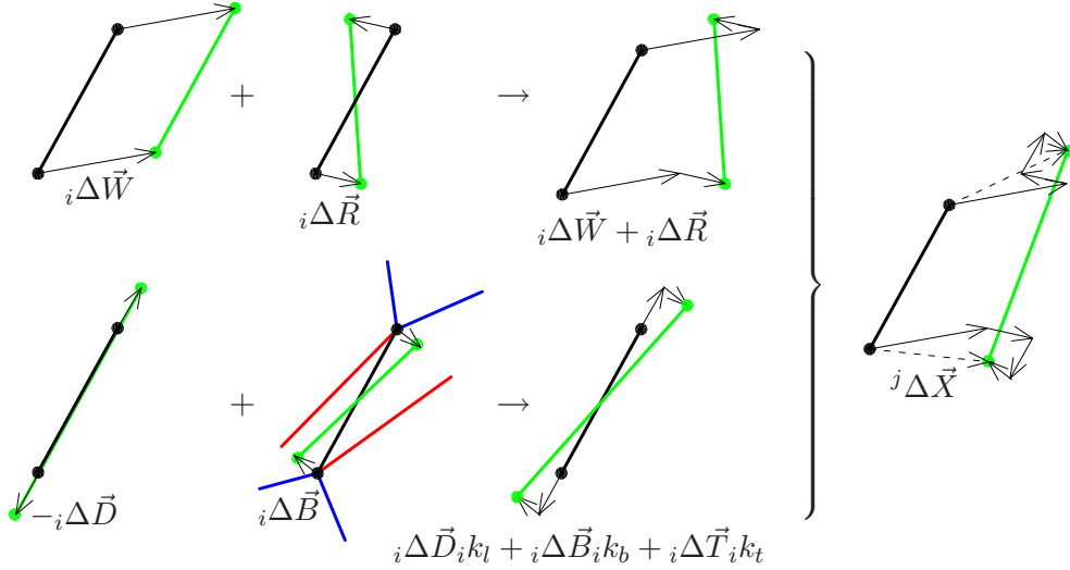
Fig. 3. General scheme to calculate displacements of elements in the Lattice Geometrical Model (torsional component i\Delta\vec{T} is not shown)
