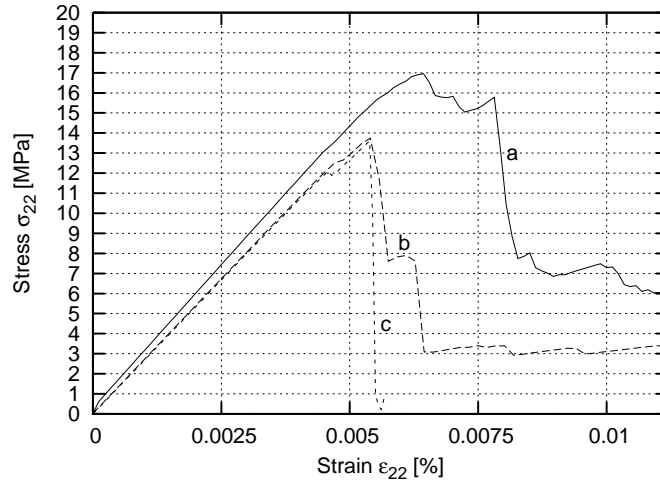
Figure 7: Effect of the ratio stiffness p = k_l/k_b on the stress–strain curve during uniaxial extension (elements were removed when local \varepsilon_{\min} = 0.02\% ): a) p=0.3 , b) p=0.025 , c) p=0.001 ( \sigma_{22} – vertical normal stress, \varepsilon_{22} – vertical normal strain)
