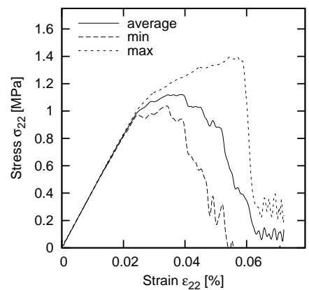
Figure 14: 2D concrete specimen subject to uniaxial extension (three-phase material) aggregate area percentage 25%, d_{50} = 3.5 mm, material parameters as in Table 1
