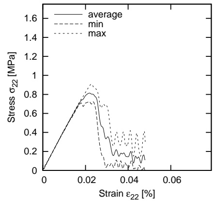
Figure 12: 2D concrete specimen subject to uniaxial extension (three-phase material), aggregate area percentage 50%, d_{50} = 3.5 mm, material parameters as in Table 1 ( \sigma_{22} – vertical normal stress, \epsilon_{22} – vertical normal strain)
