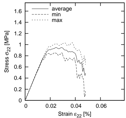
Figure 13: 2D concrete specimen subject to uniaxial extension (three-phase material) aggregate area percentage 50%, d_{50} = 12 mm, material parameters as in Table 1
