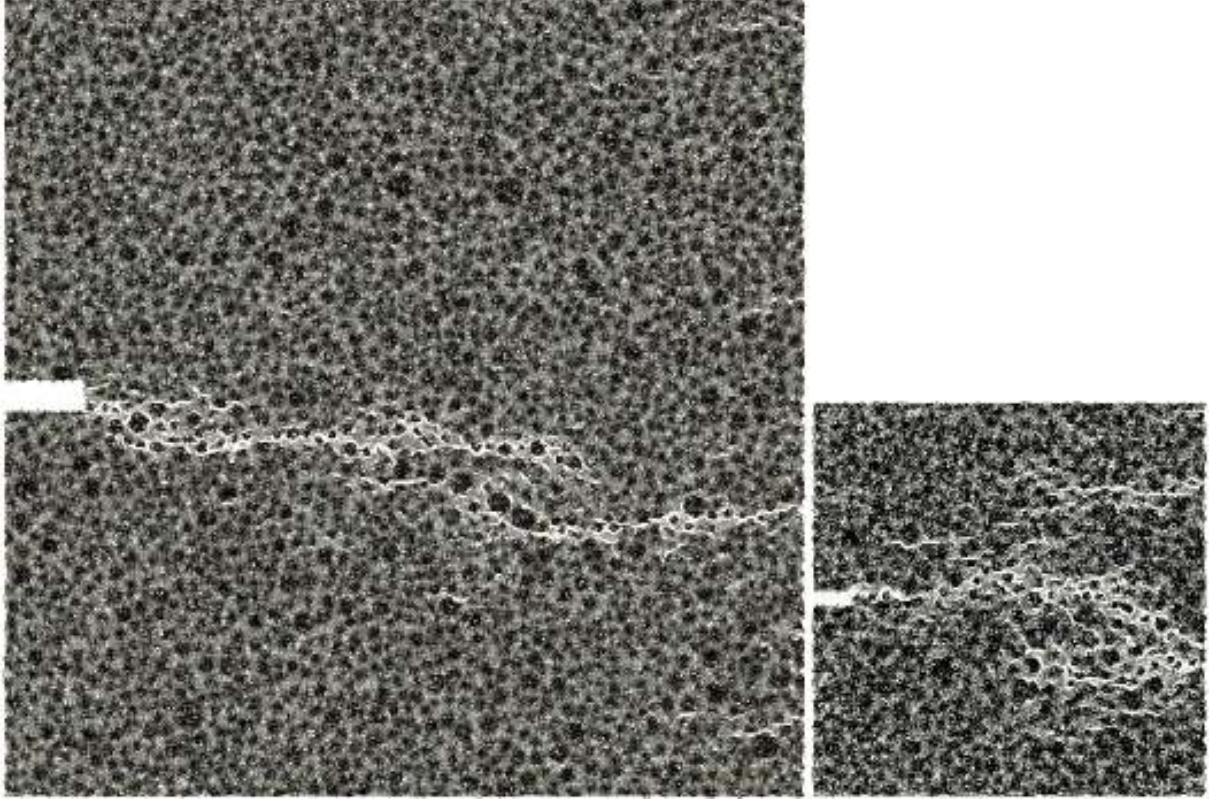
Figure 18: Fracture in 2 concrete specimens of different size ( 20 \times 20 \text{ cm}^2 and 10 \times 10 \text{ cm}^2 )
