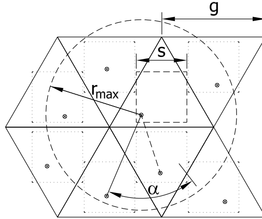
Figure 2: Scheme to assume a non-uniform distribution of beams in the lattice ( s – size of interior squares, r_{\max} – maximum beam radius, \alpha – minimum angle between two beams, g – size of triangular grid)
