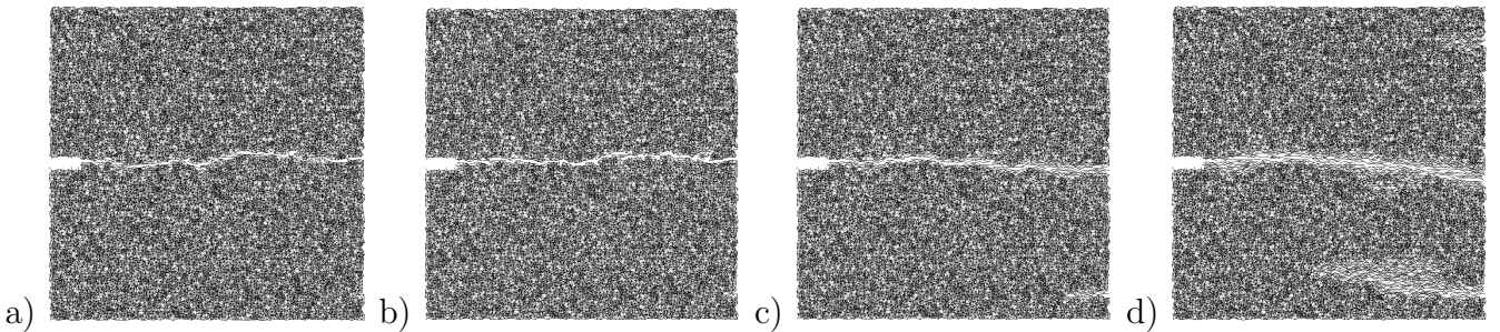
Figure 9: Effect of the characteristic length l_c on the fracture process (elements were removed when local \varepsilon_{\min} = 0.02\% , p = 0.6 ): a) l_c = 0 (local approach), b) l_c = g , c) l_c = 2g , d) l_c = 3g (non–local approach)
