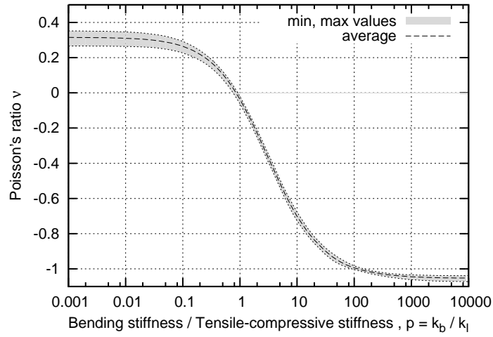
Figure 4: Influence of the ratio between the bending and longitudinal stiffness p = k_b/k_l on Poisson's ratio \nu during uniaxial compression with smooth edges (using semi-logarithmic scale)
