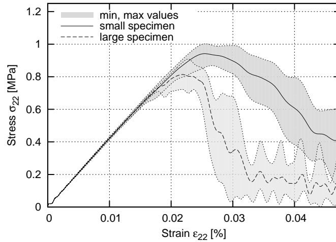
Figure 16: Deterministic size effect for 2D concrete specimens subject to uniaxial extension with sizes 10 \times 10 cm 2 and 20 \times 20 cm 2 , aggregate area percentage 50%, d_{50} = 3.5 mm, material parameters as in Table 1
