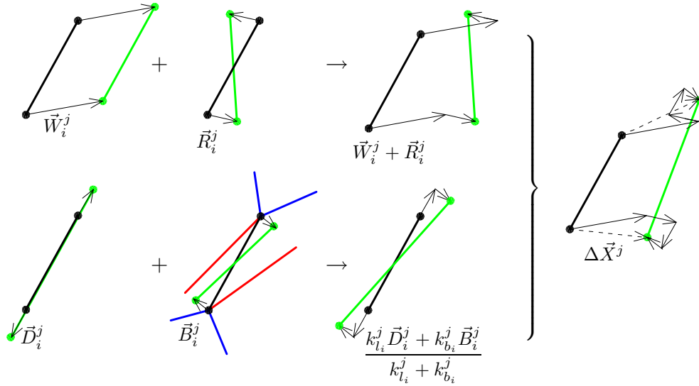
Figure 3: General scheme to calculate displacements of elements in the lattice
