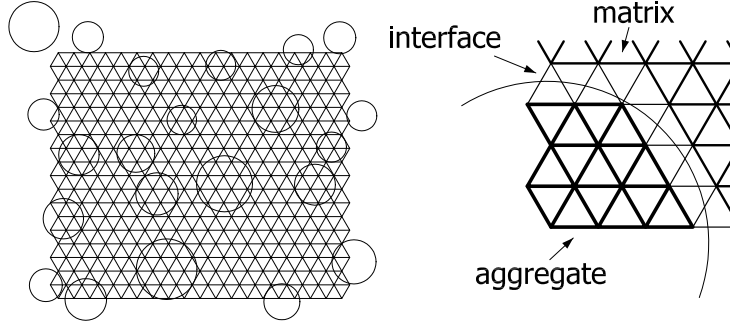
Figure 1: Lattice of beams for concrete consisting of aggregate, cement matrix and interface [44]
