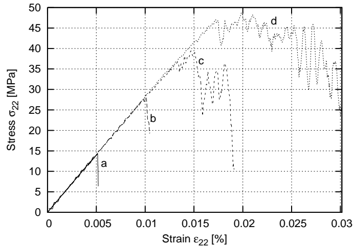
Figure 8: Effect of the characteristic length on the stress–strain curve ( p=0.6 , specimen 100 \times 100 \text{ mm}^2 ): a) l_c=0 (local approach), b) l_c = g , c) l_c = 2g , d) l_c = 3g (non–local approach, \sigma_{22} – vertical normal stress, \varepsilon_{22} – vertical normal strain)
