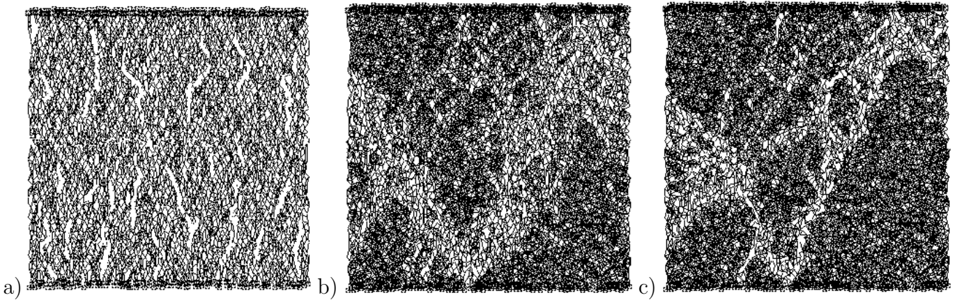
Figure 6: Effect of the stiffness ratio p = k_b/k_l between the bending and longitudinal stiffness on the crack pattern during uniaxial compression with smooth edges (elements were removed when local \epsilon_{\min} = 0.02\% ): a) p = 0.3 , b) p = 0.01 , c) p = 0.001
