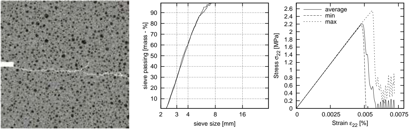
Figure 11: 2D specimen subject to uniaxial extension (two-phase material): cement matrix: p_m = k_b/k_l = 0.7 (with k_l = 0.1 ), local \varepsilon_{\min} = 0.02\% and aggregate: p_a = k_b/k_l = 0.7 (with k_l = 0.3 ), local \varepsilon_{\min} = 0.0133\%
