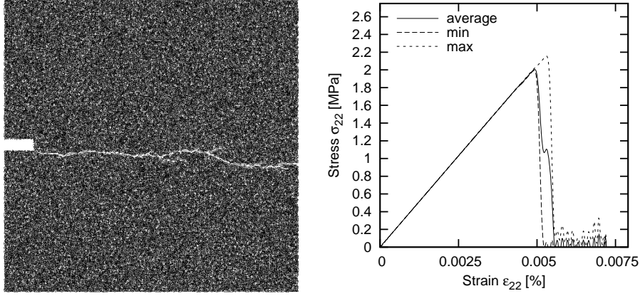
Figure 10: 2D specimen subject to uniaxial extension (one-phase material): p = k_b/k_l = 0.7 (with k_l = 0.1 ) and local \varepsilon_{\min} = 0.02\%
