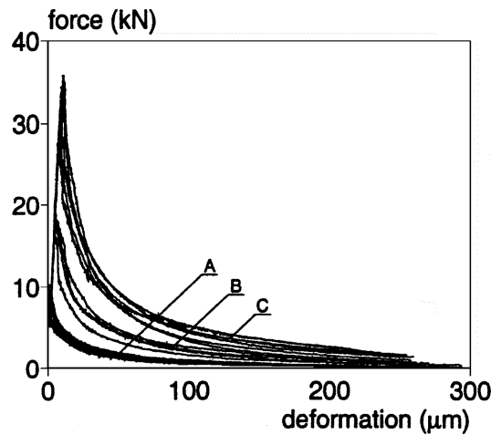
Figure 17: Experimental force-deformation diagram for 3 different dog-bone shaped specimens h \times b : A) 75 \times 50 mm 2 , B) 150 \times 75 mm 2 , C) 300 \times 200 mm 2 [46] ( h - height, b - width)
