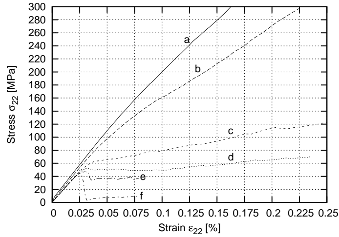
Figure 5: Effect of the stiffness ratio p = k_b/k_l between the bending stiffness and longitudinal stiffness on the stress-strain curve during uniaxial compression with smooth edges (elements were removed when local \epsilon_{\min} = 0.02\% ): a) p = 0.6 , b) p = 0.3 , c) p = 0.06 , d) p = 0.025 , e) p = 0.01 , f) p = 0.001 ( \sigma_{22} – vertical normal stress, \epsilon_{22} – vertical normal strain)
