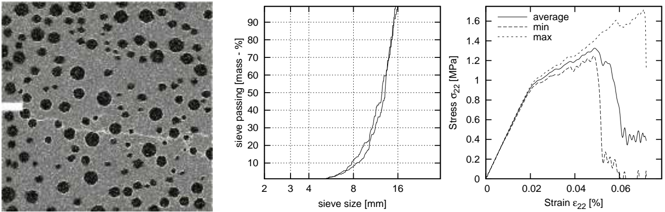
Figure 15: 2D concrete specimen subject to uniaxial extension (three-phase material) aggregate area percentage 25%, d_{50} = 12 mm, material parameters as in Table 1
