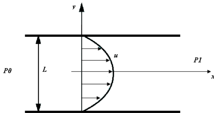
Figure1.1: Poiseuille flow
