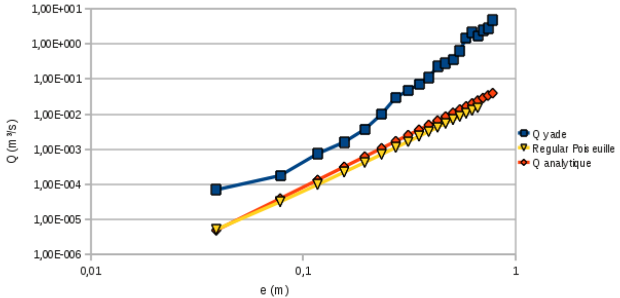
Figure 3.22: Numerical and analytical flows as functions of e .
