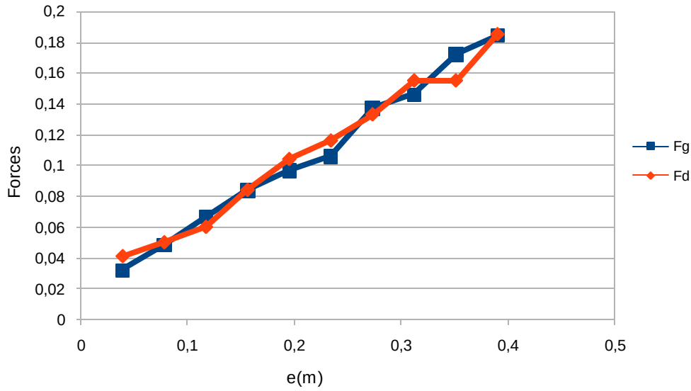
Figure 3.18: Fluid forces on particles in the right and left side of the trench as functions of e .
